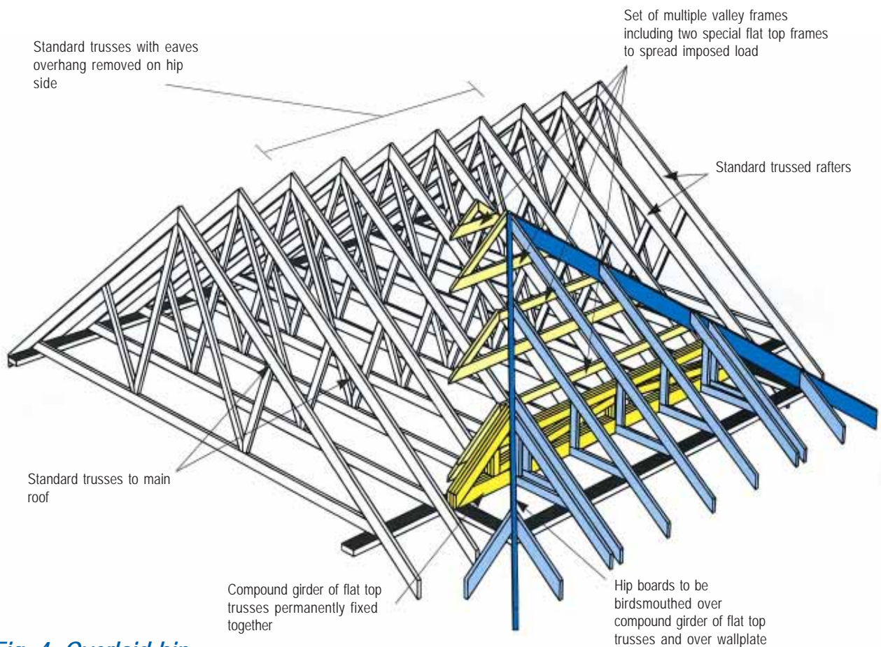
Fig. 4 Overlaid hip
