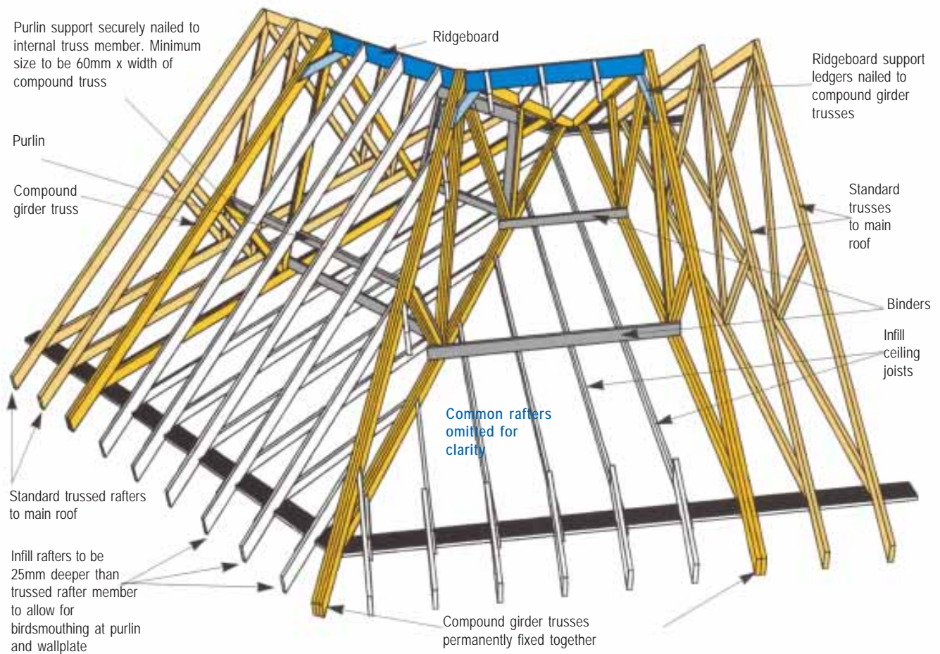
Fig. 5 Dogleg intersection
