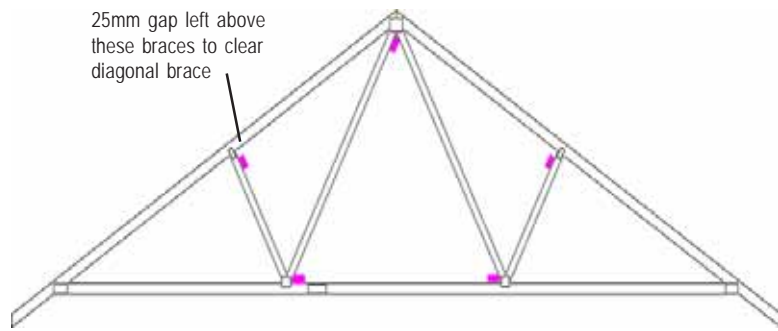
Fig. 2 Positions of longitudinal braces
