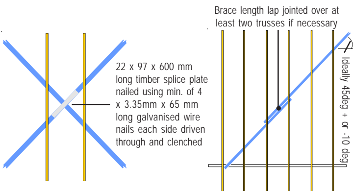
Fig. 7 Splicing of intersecting diagonal braces and end jointing
