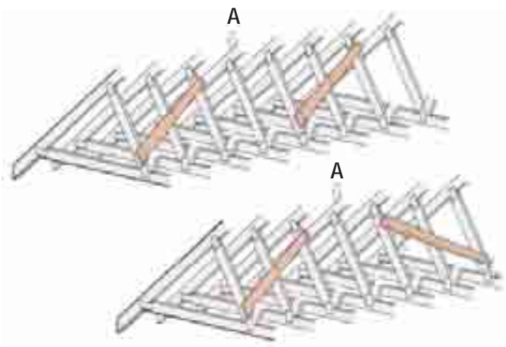
Fig. 8 Alternative fixing arrangement for chevron braces (truss span over 8m)
