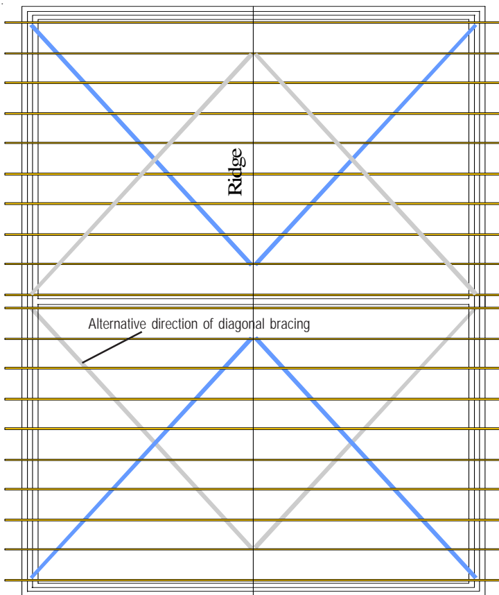
Fig. 6 Plan of rafter diagonal bracing arrangement on a wide fronted roof
