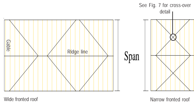
Fig. 5 Plan of rafter diagonal bracing on differing plan shapes
