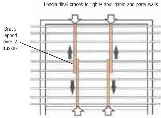
Fig. 3 The fixing of longitudinal braces
