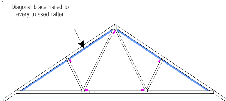
Fig. 4 Position of diagonal wind braces
