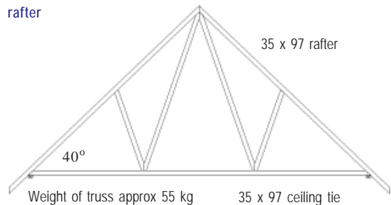
Fig. 1 Typical 8 metre span conventional trussed rafter
