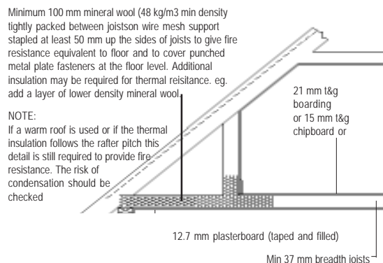
Fig. 11 Requirements of TRADA Approved Document
