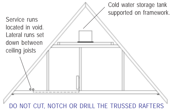
Fig. 6 Services in trussed rafter roofs
