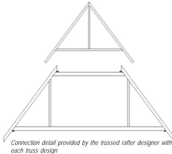
Fig. 5 Two-part 'RiR' trussed rafters
