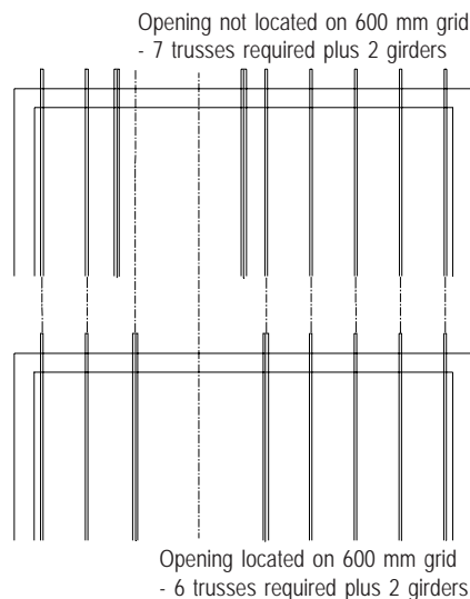
Fig. 7 Positioning of trussed rafters
