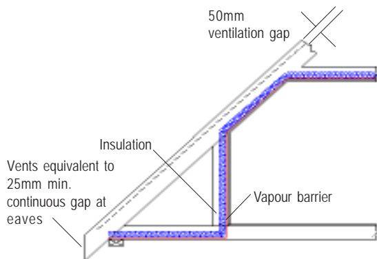
Fig. 9 Roof insulation
