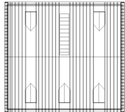
Suitable layout - since staircase parallel to trusses, windows directly opposite and small widths may be site framed
