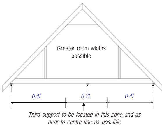
Fig. 3 Three bearing 'RiR' trussed rafter
