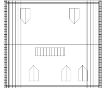
Unsuitable layout - impossible to provide 'RiR' trusses to support this roof since windows and stairs all overlap.
