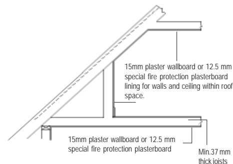
Fig. 12 Alternative solution
